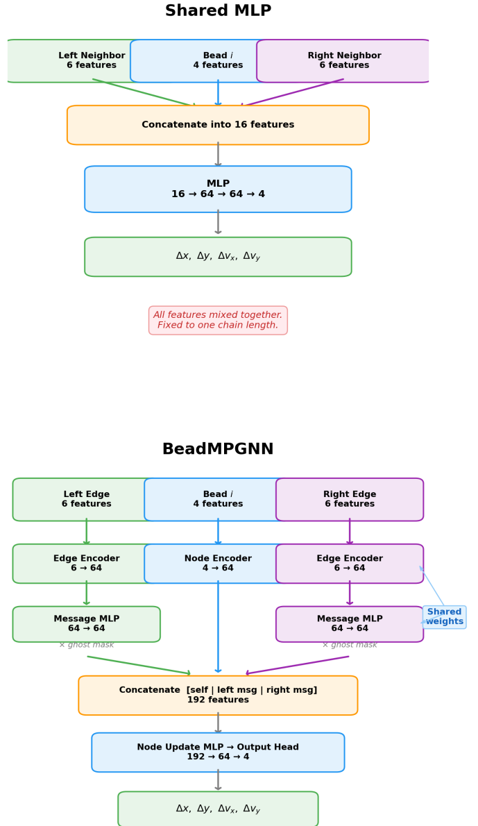
Fig. 1: Top: the shared MLP concatenates all 16 features into a single vector. Bottom: the BeadMPGNN encodes node and edge features separately, computes messages per edge, applies ghost masking for missing neighbors, and concatenates the results before the node update.
