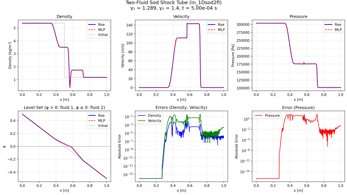
Figure 11: Two-fluid Sod shock tube: MLP vs analytical Roe. The model handles the interface between gases with different \gamma values seamlessly.
