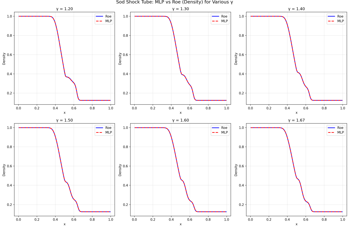
Figure 12: Density profiles for Sod shock tubes with different \gamma values. Blue solid: analytical Roe; red dashed: MLP. All six cases show excellent agreement.
