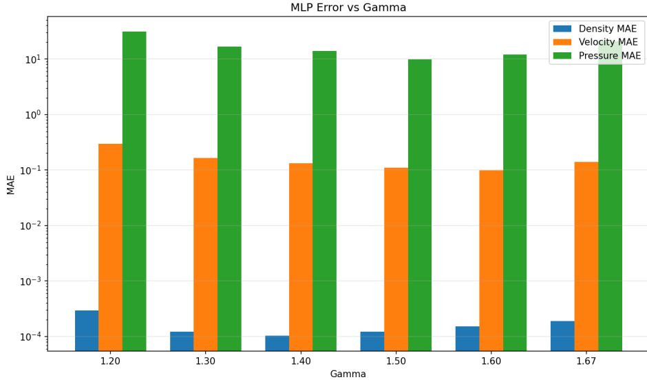
Figure 13: Error summary across gamma values. Best performance is in the middle of the training range ( \gamma = 1.4 – 1.5 ), with slightly higher errors at the edges.
