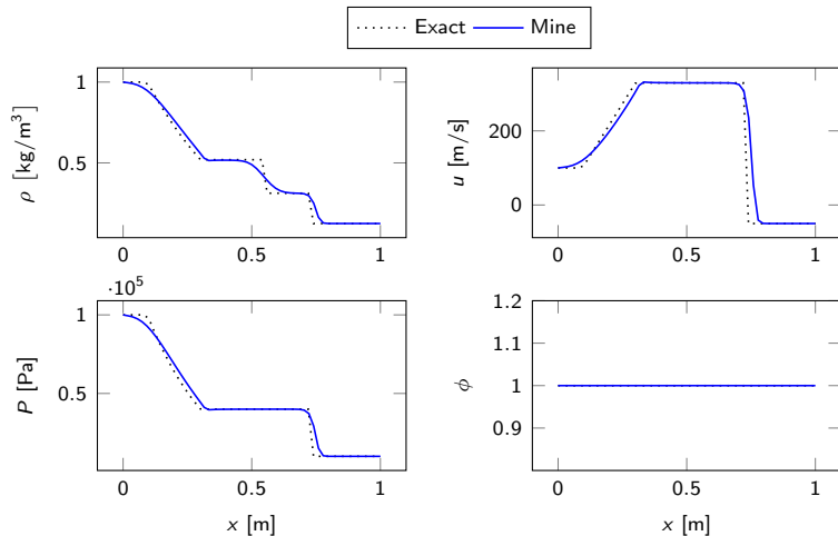
Figure: Shock tube problem results at t = 5 \times 10^{-4} s
