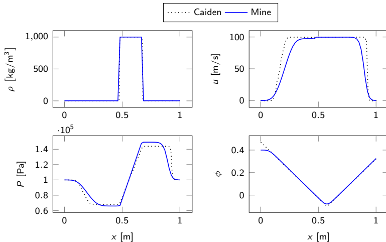
Figure: GFM results of 1D example 1 at t = 7.5 \times 10^{-4} s
