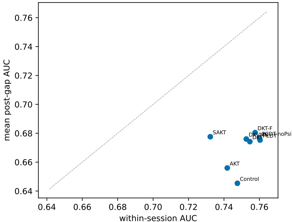
assismments_2021 seed 20260203 — corrected DKVMN
