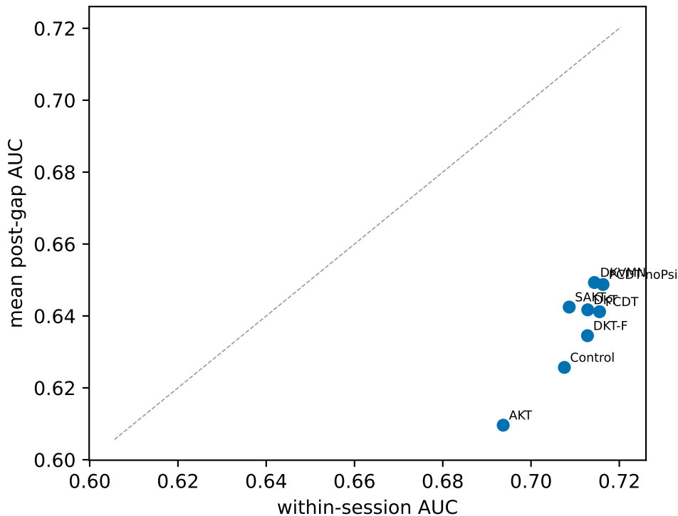
ednet_flat seed 20260202 — corrected DKVMN
