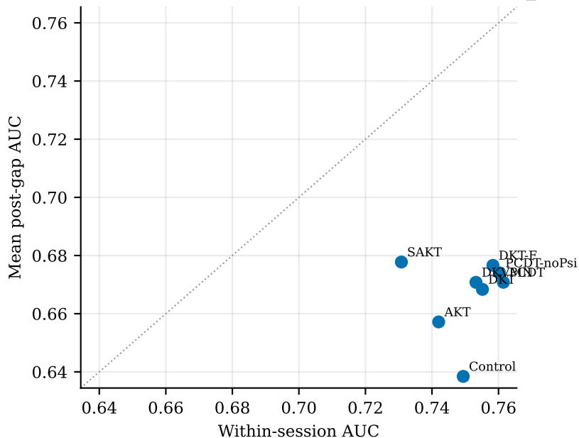
Within-session vs post-gap performance (assistsments_2021)
