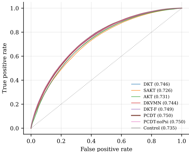
ROC — all eight models (assistments_2021)
