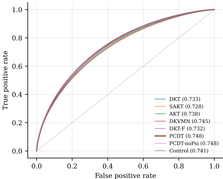
ROC — all eight models (junyi)
