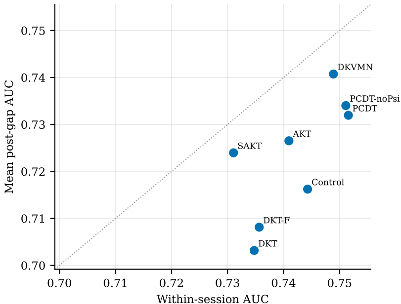
Within-session vs post-gap performance (junyi)
