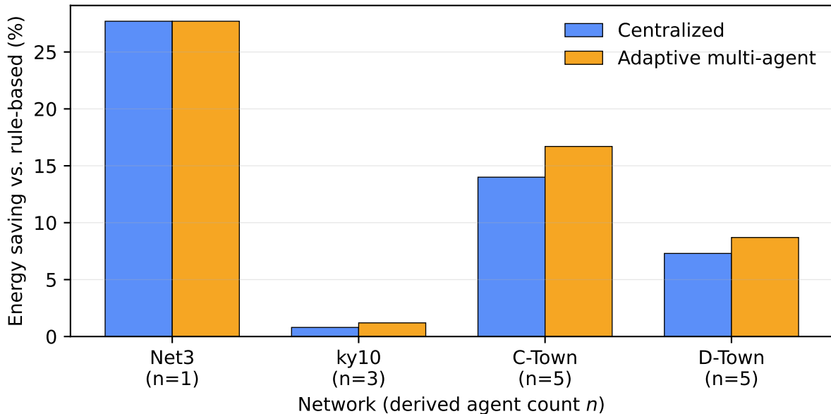
Cross-network energy savings at held demand satisfaction
