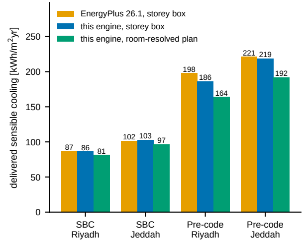
Figure 5: Like-for-like comparison with EnergyPlus 26.1: delivered sensible cooling under ideal control at the reference setpoints. On the same storey-box geometry the two programs agree within a few per cent; the room-resolved plan delivers less, because its passive rooms float above the setpoint.
