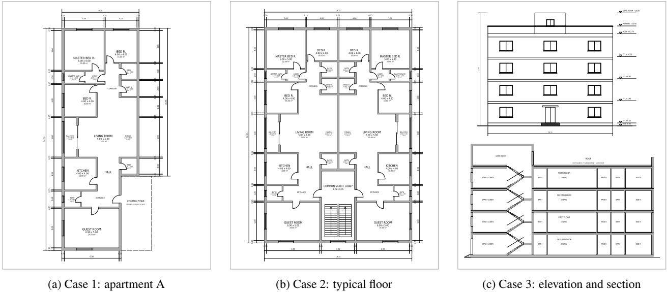
Figure 3: The building analysed in the three cases (drawings generated as layered DXF files; clear dimensions in metres). (a) Apartment A, analysed alone in Case 1. (b) The typical floor: two mirror-image apartments around the common stair; north is up. (c) South elevation (top) and section A–A through the stair (bottom) of the four-storey building (floor-to-floor height 3.40 m, 3.00 m clear; windows from 0.90 to 2.40 m above each floor). The zone rectangles of the model follow the wall centrelines of (b).
