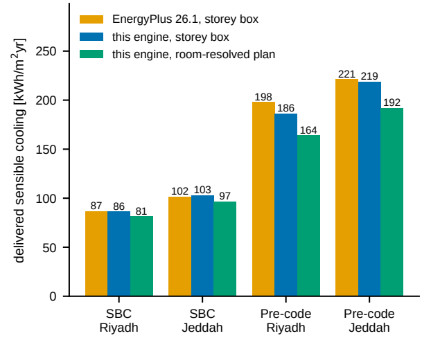
Figure 5: Like-for-like comparison with EnergyPlus 26.1: delivered sensible cooling under ideal control at the reference setpoints. On the same storey-box geometry the two programs agree within a few per cent; the room-resolved plan delivers less, because its passive rooms float above the setpoint.
