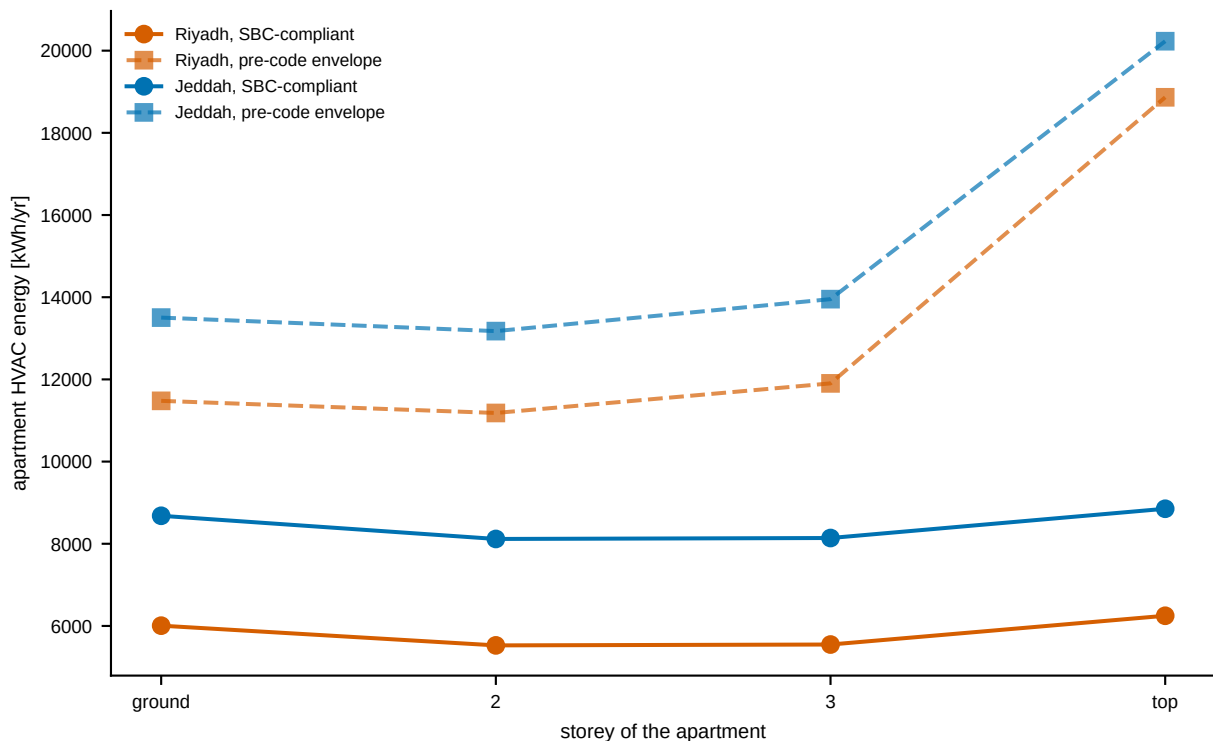
Apartment energy by storey in the four-storey building
