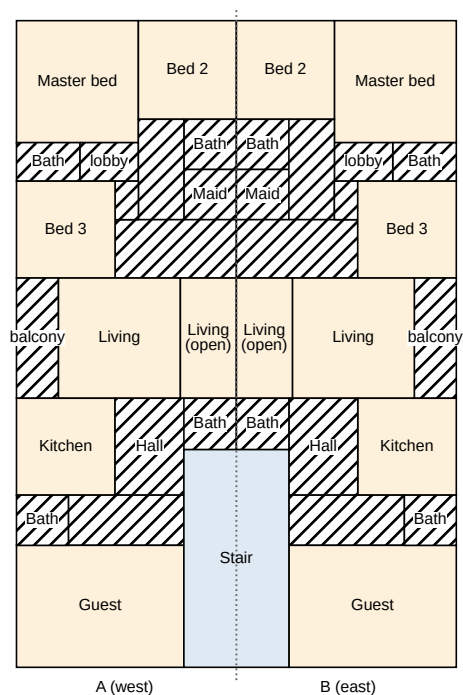
(b) Case 2: typical floor (19.15 m × 28 m)
