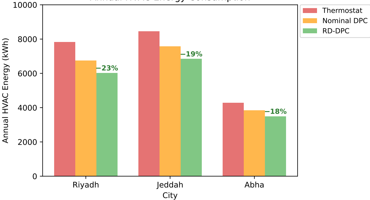
Annual HVAC Energy Consumption
