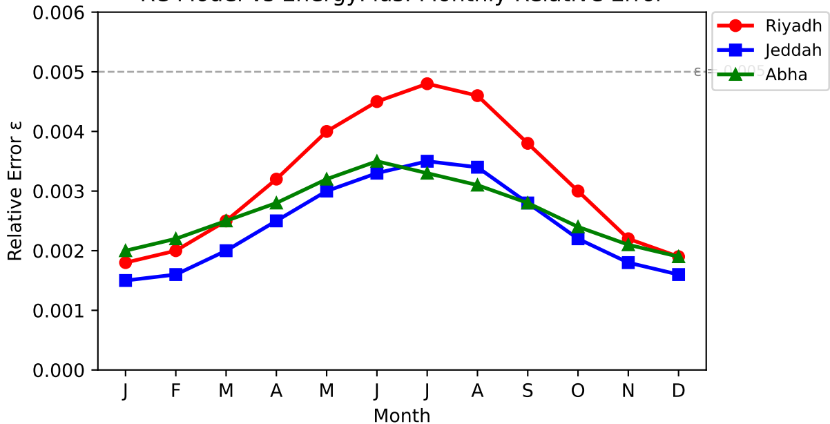
RC Model vs EnergyPlus: Monthly Relative Error
