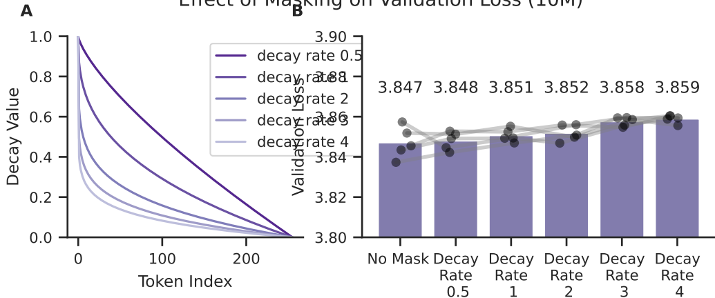
Effect of Masking on Validation Loss (10M)
