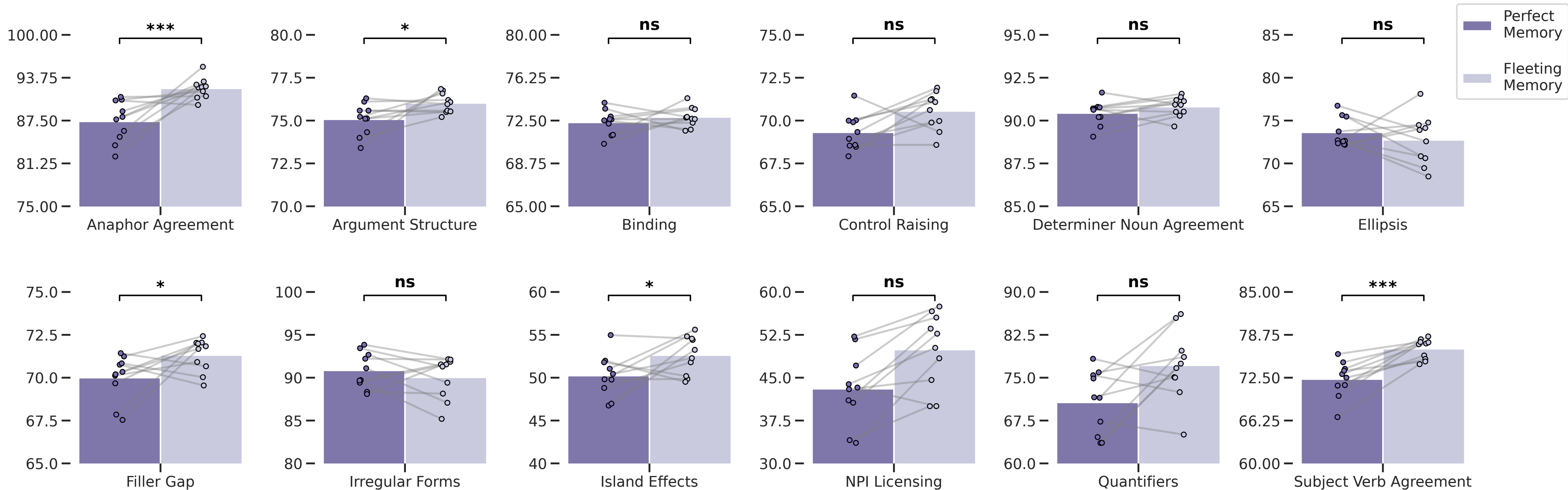
BLIMP Subtask Score (100M)
