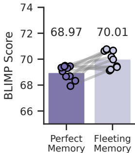
B) BLIMP Score
