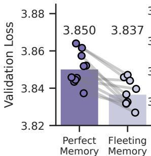
A) Validation Loss
