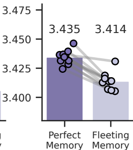
A) Validation Loss
