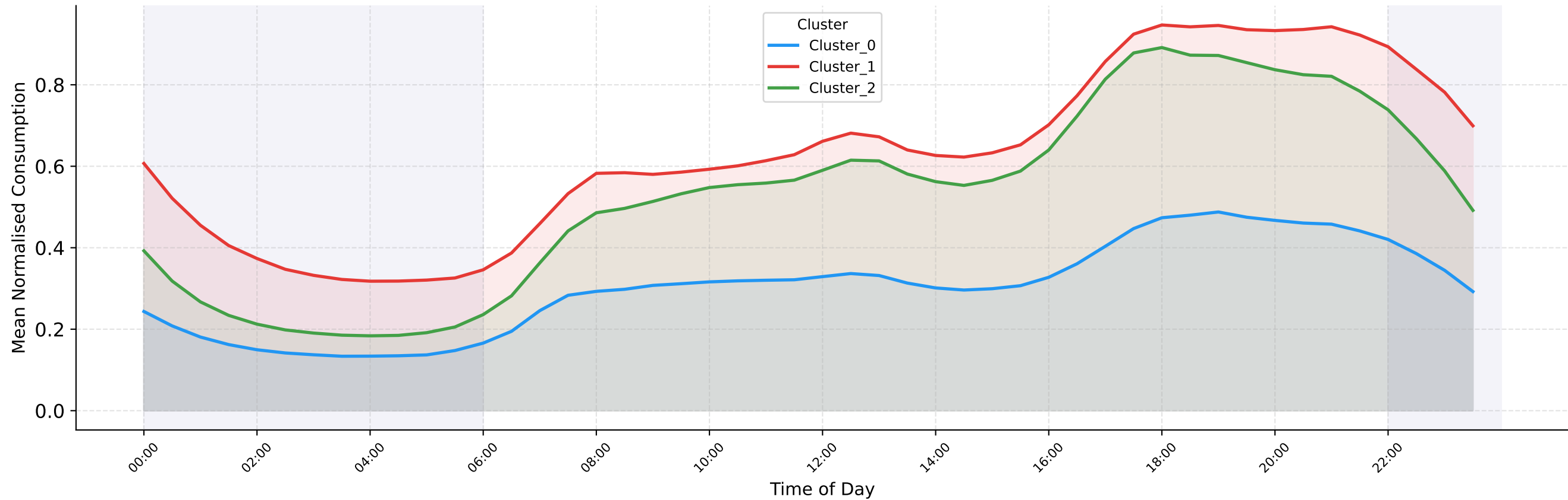
Intraday Consumption Profile (24h) — Irish_Best_K3 Dataset
