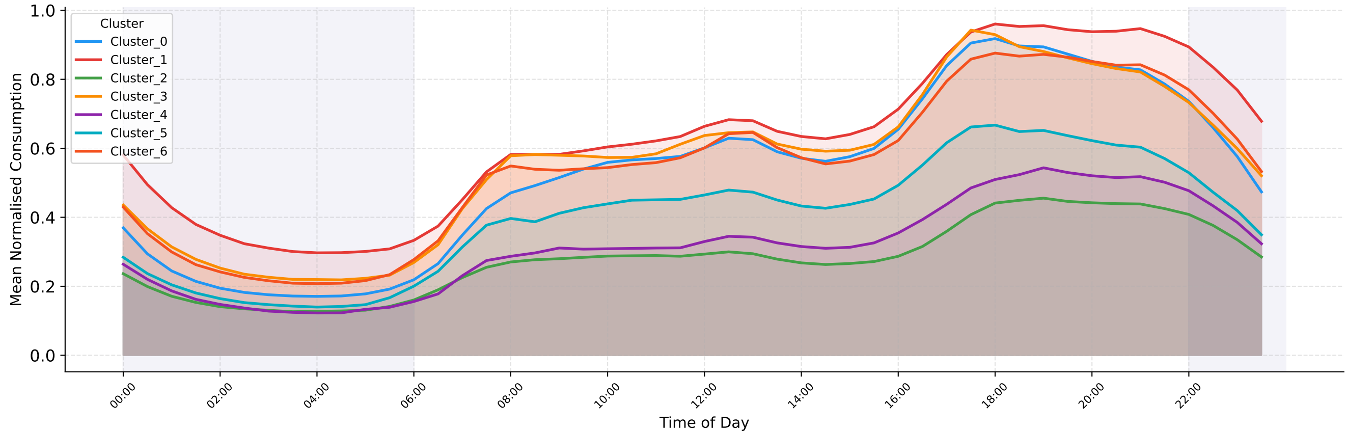
Intraday Consumption Profile (24h) — Irish_Worst_K7 Dataset
