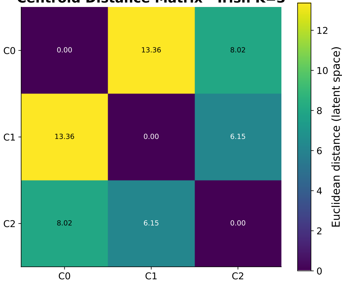
Centroid Distance Matrix - Irish K=3
