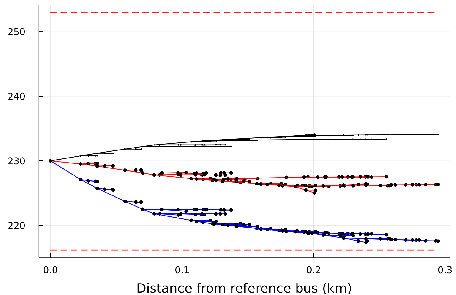
EV (7 kW, 1 \phi ): voltage drop
