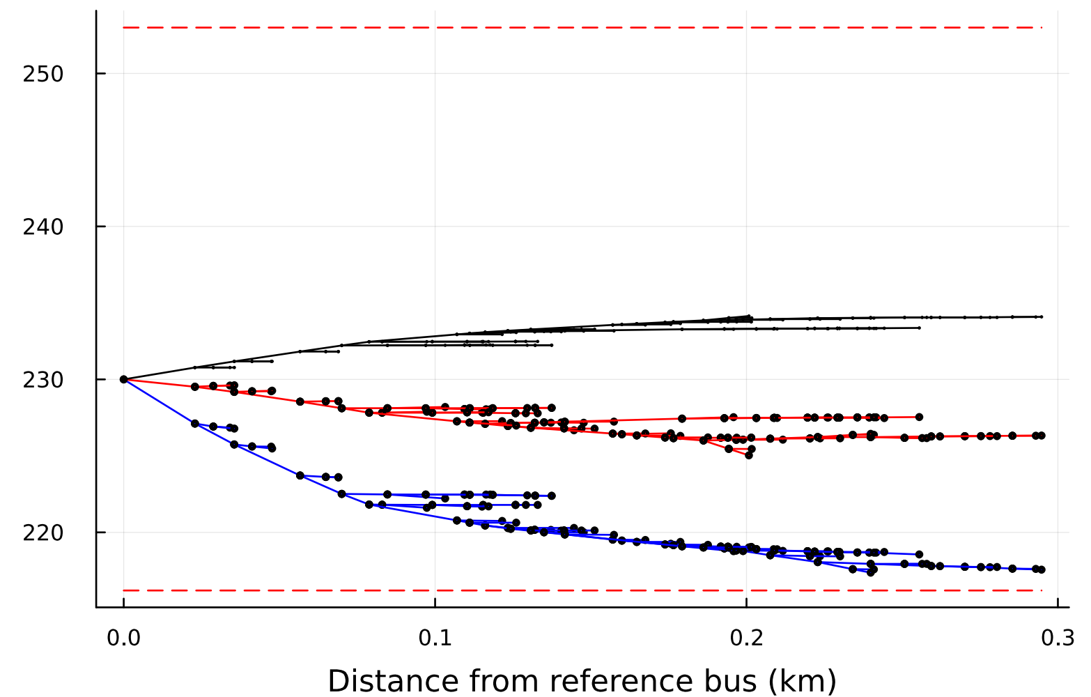
twoev_distributed_mid_plus_weakest: voltage profile
