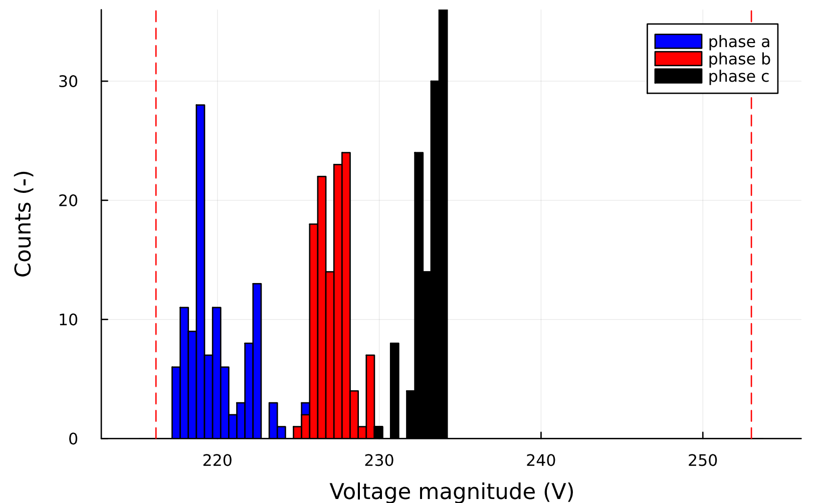
twoev_distributed_mid_plus_weakest: voltage histogram
