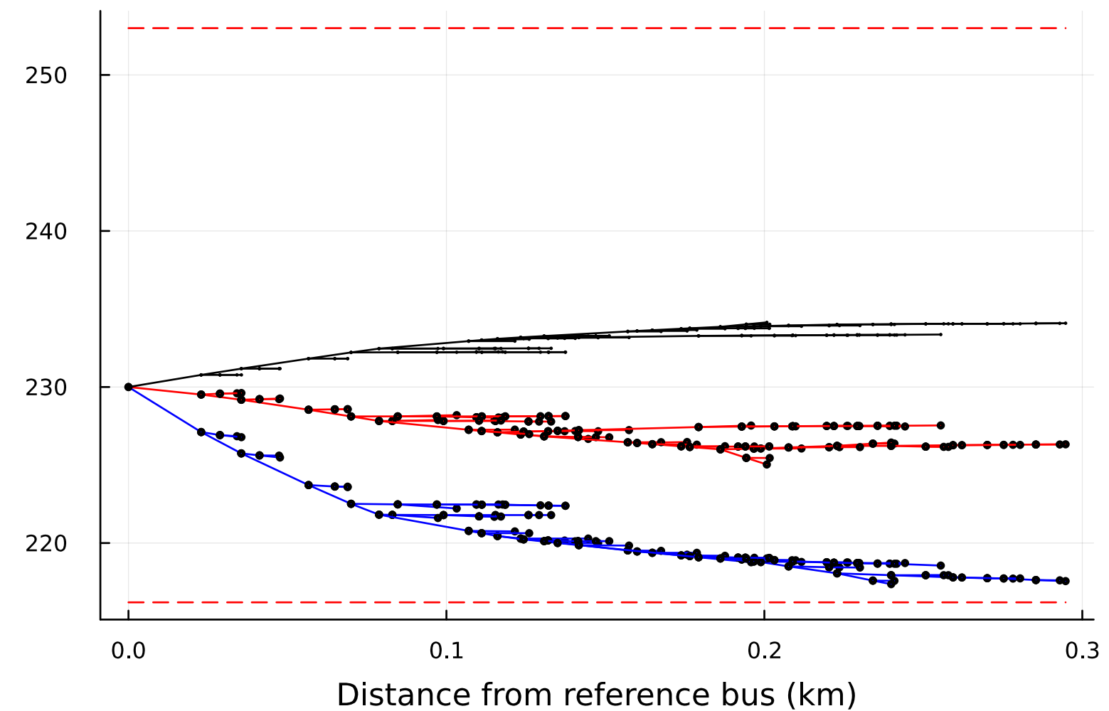
twoev_clustered_samephase: voltage profile
