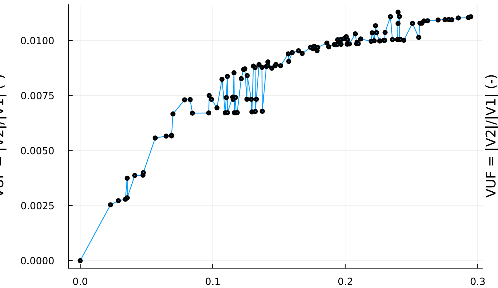
Distance from reference bus (km) Compare VUF: baseline vs ev_far
