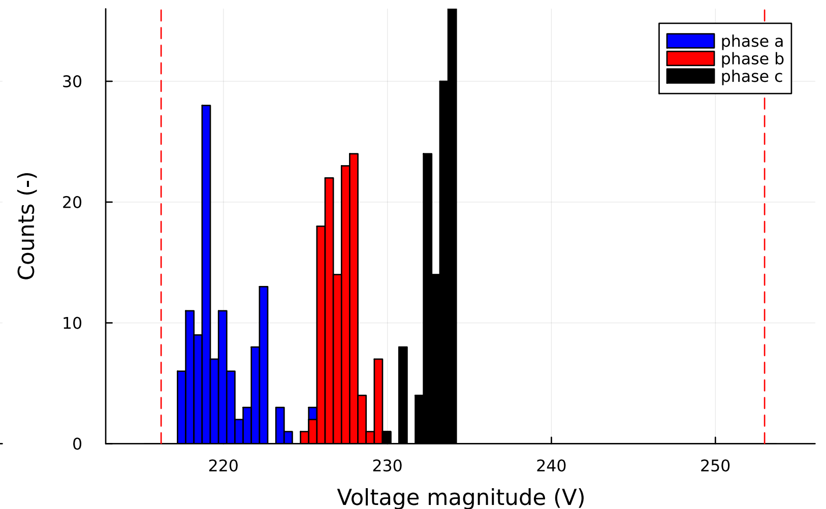
twoev_clustered_samephase: voltage histogram
