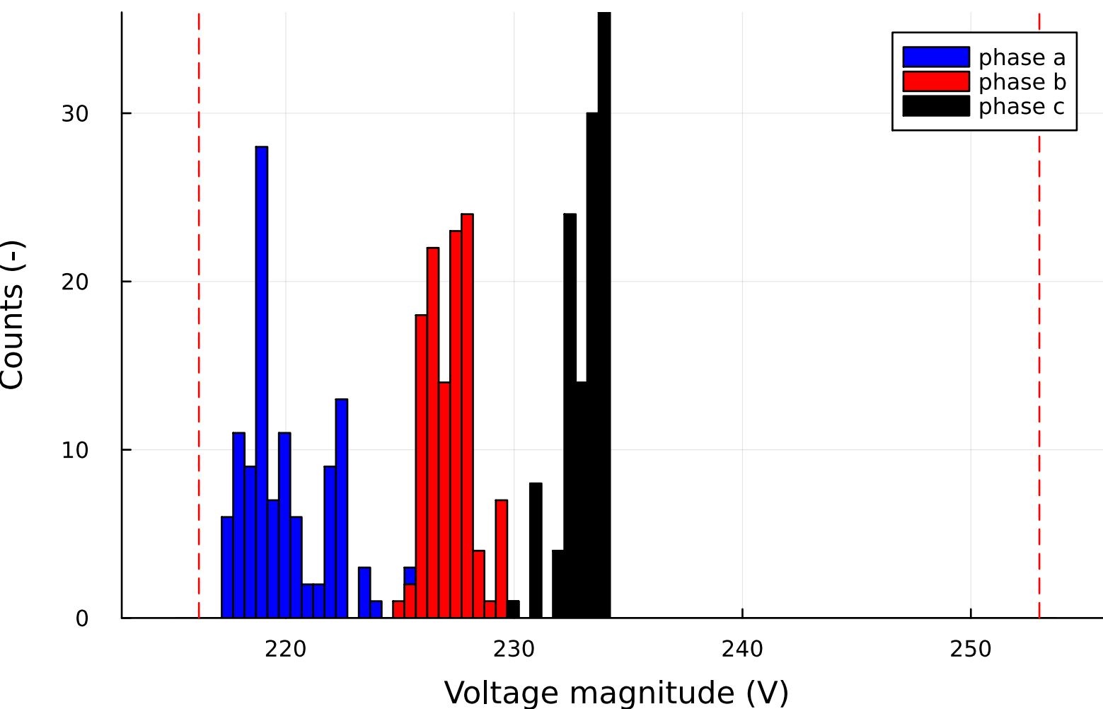
Baseline: voltage histogram
