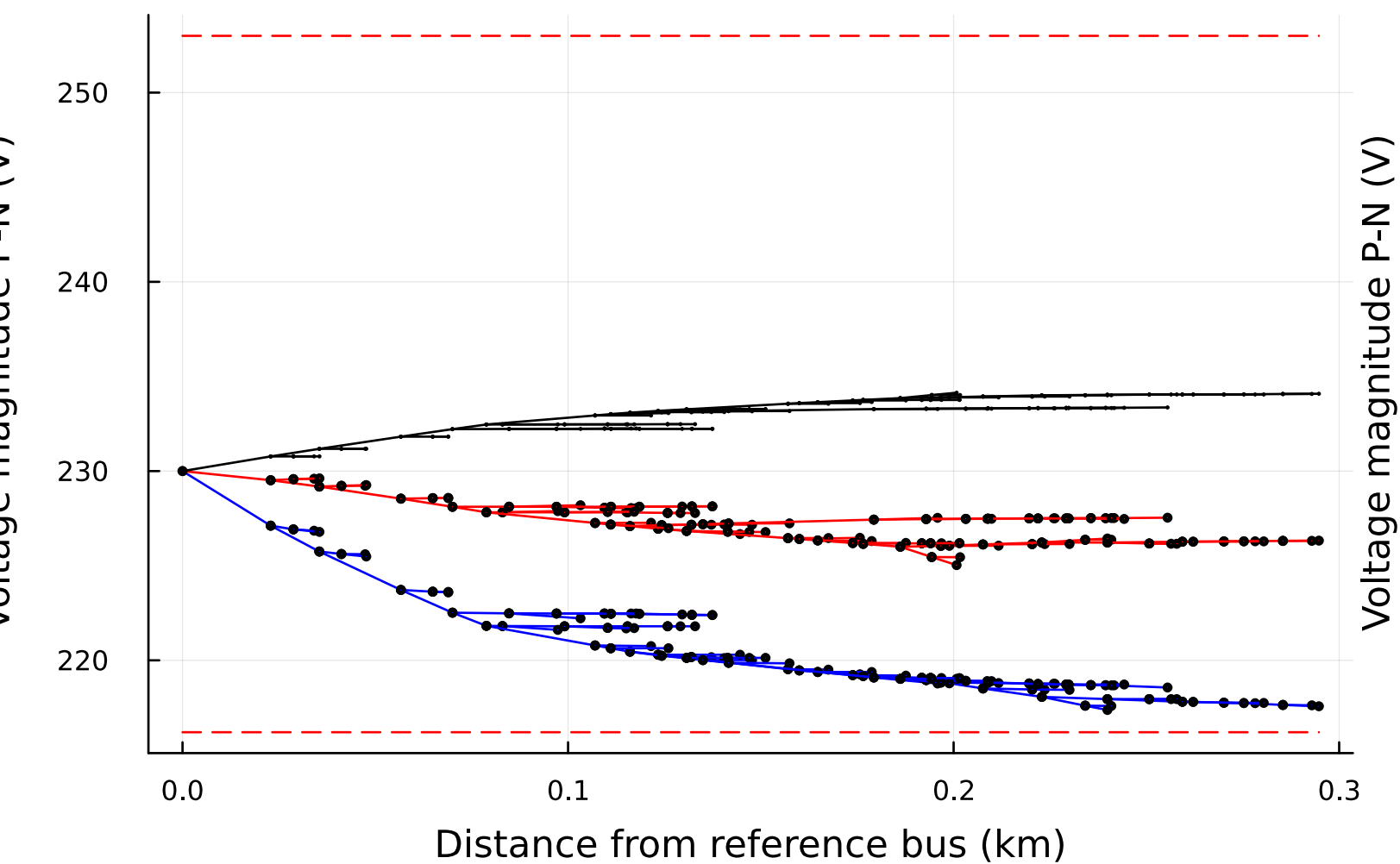
Baseline: voltage drop
