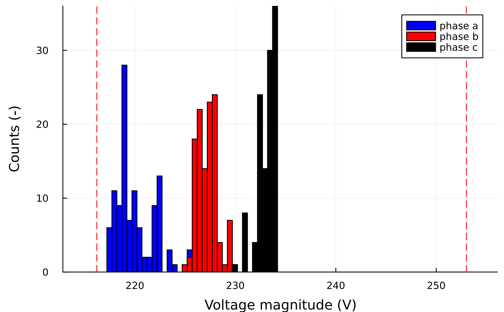
EV (7 kW, 1 \phi ): voltage histogram
