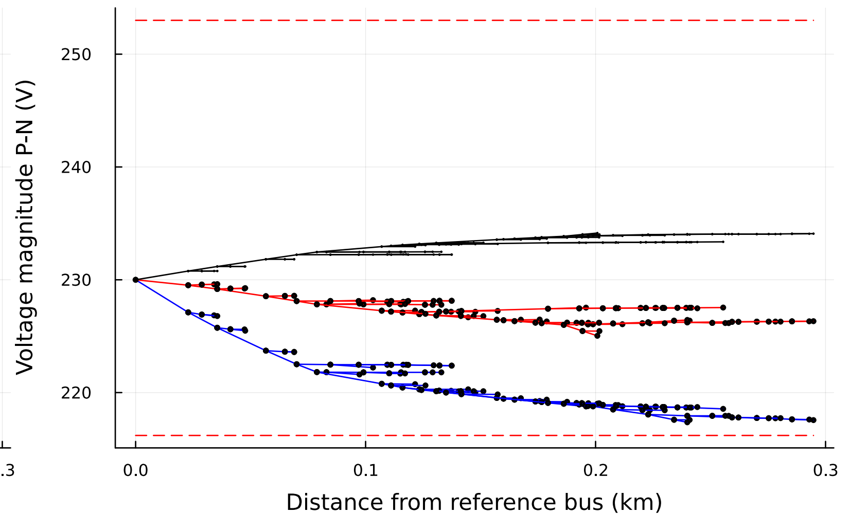
twoev_distributed_source_plus_weakest: voltage profile
