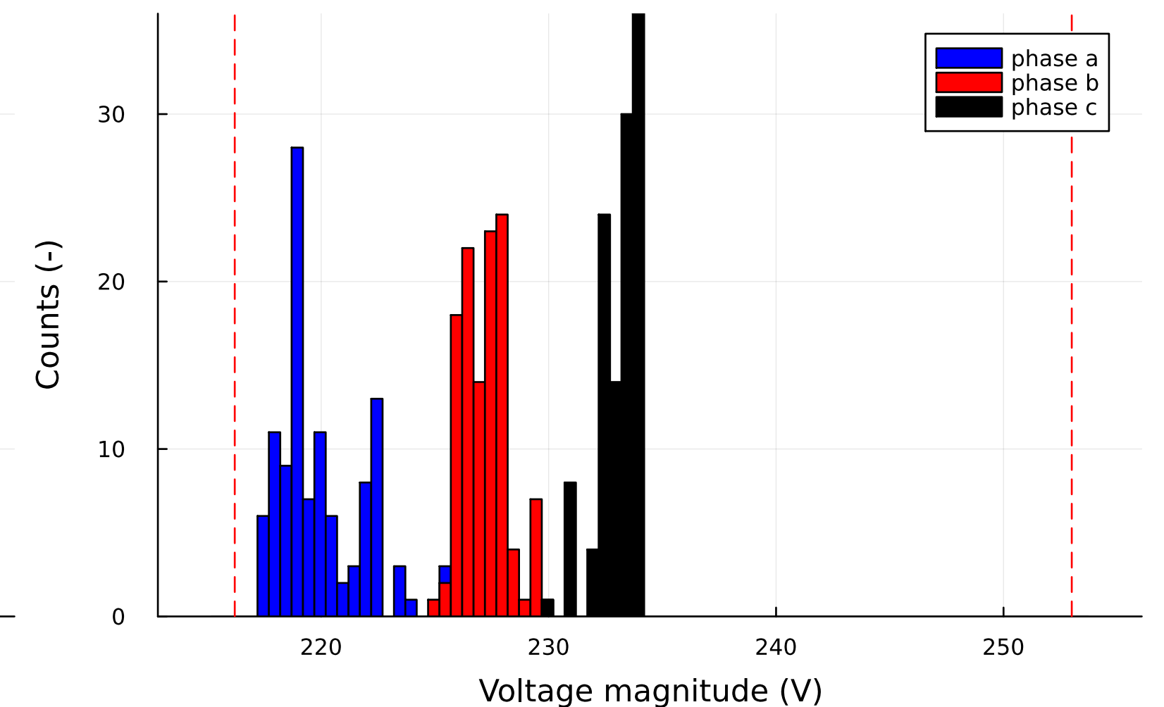
twoev_distributed_source_plus_weakest: voltage histogram
