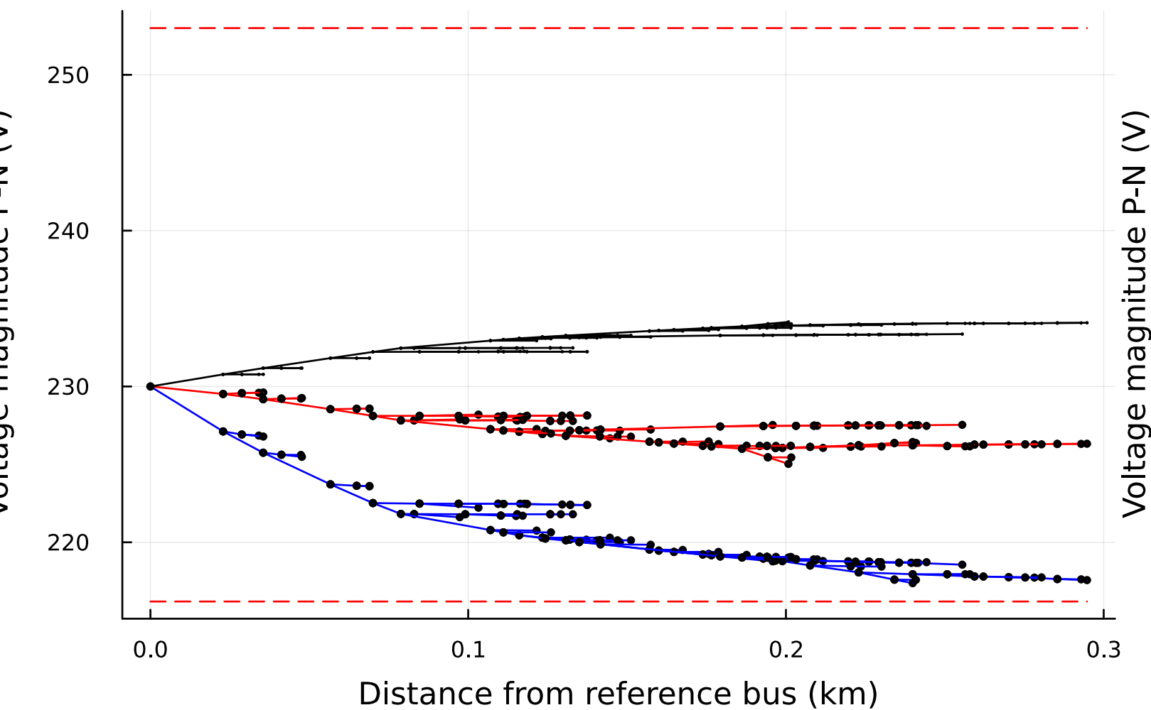
Baseline: voltage profile
