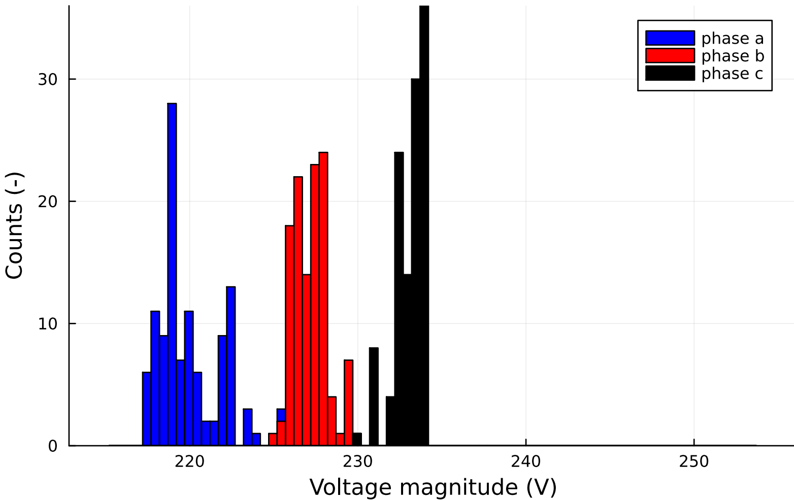
Voltage histogram
