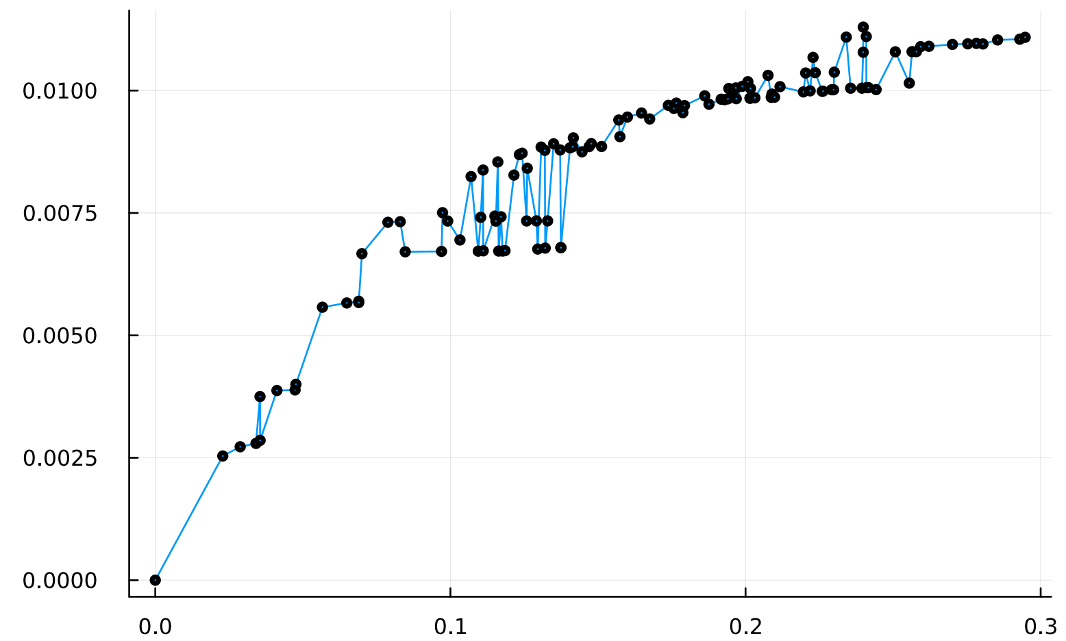
Distance from reference bus (km) Compare VUF: baseline vs ev_far
