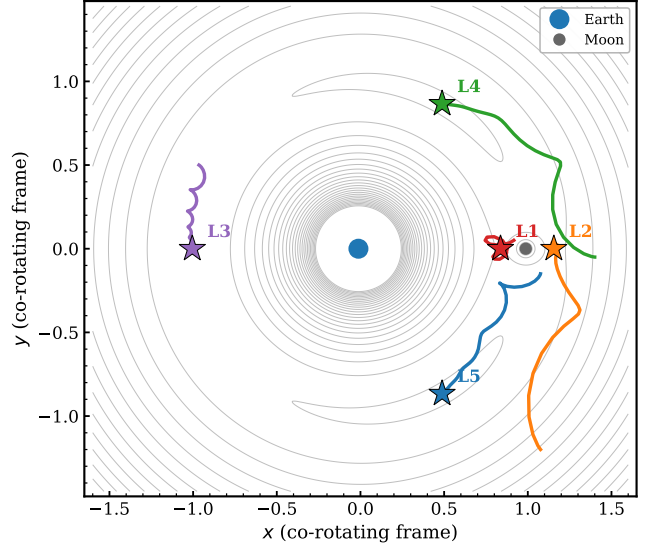
FIG. 3. Representative memory-as-dissipation trajectories for Earth–Moon ( \mu = 0.0121 ), one per Lagrange point, from a 10 \times 10 grid of starts. Grey curves: level sets of \Omega . Stars: the discovered equilibria. No solution coordinates are supplied to the integrator.
