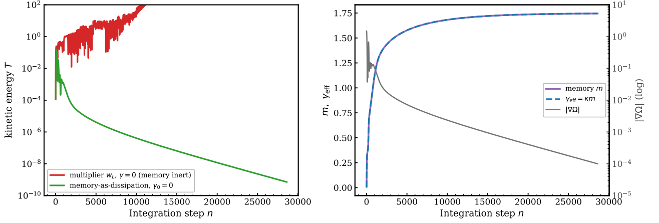
FIG. 2. Why the memory now computes, for one representative initial condition with no external damping. Left: kinetic energy T = \frac{1}{2} \|\dot{\mathbf{r}}\|^2 (log scale). Under the multiplier ansatz (7)–(9) with \gamma = 0 (red), T remains \mathcal{O}(1) and grows—the memory cannot dissipate (Proposition 1). Under memory-as-dissipation (13a)–(13d) with \gamma_0 = 0 (green), T \rightarrow 0 . Right: for the green run, the memory m (solid) and the damping \gamma_{\text{eff}} = \kappa m (dashed) ratchet up from zero and saturate, while the clause violation \|\nabla\Omega\| (grey, right axis) decays to the threshold.
