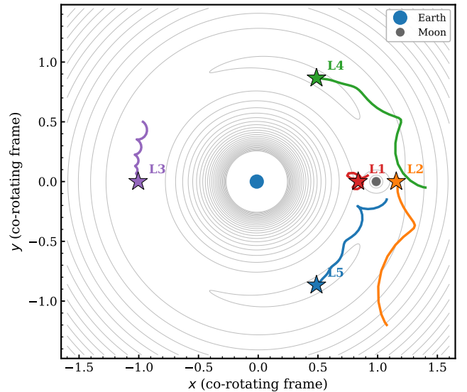
Figure 3: Representative memory-as-dissipation trajectories for Earth–Moon ( \mu = 0.0121 ), one per Lagrange point, from a 10 \times 10 grid of starts. Grey curves: level sets of \Omega . Stars: the discovered equilibria. No solution coordinates are supplied to the integrator.
