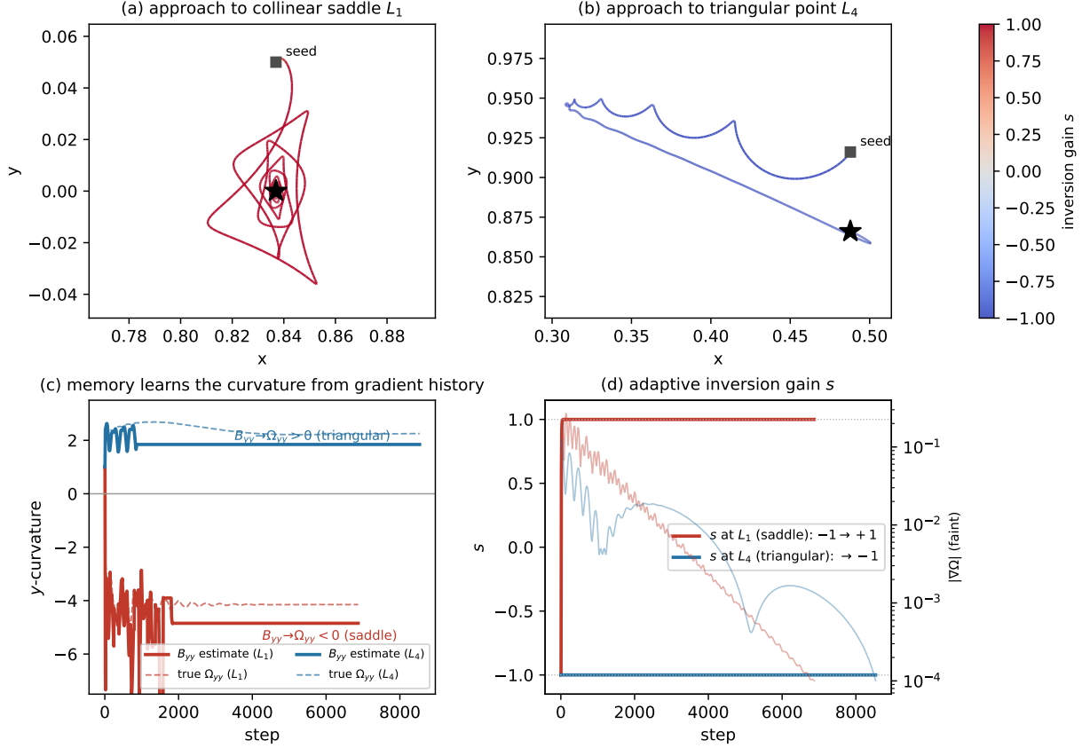
FIG. 2. The memory learns the curvature. Two Earth–Moon trajectories of the same Hessian-free machine. (a),(b) phase-plane paths coloured by the inversion gain s : red ( s \rightarrow +1 ) on the approach to the collinear saddle L_1 , blue ( s \rightarrow -1 ) on the approach to the triangular minimum L_4 . (c) the quasi-Newton estimate B_{yy} (solid) tracks the true \Omega_{yy} (dashed) from gradient history alone—negative at the saddle, positive at the minimum. (d) the gain s responds to what was learned: -1 \rightarrow +1 at the saddle, held at -1 at the minimum, while \|\nabla\Omega\| (faint) decays to convergence.
