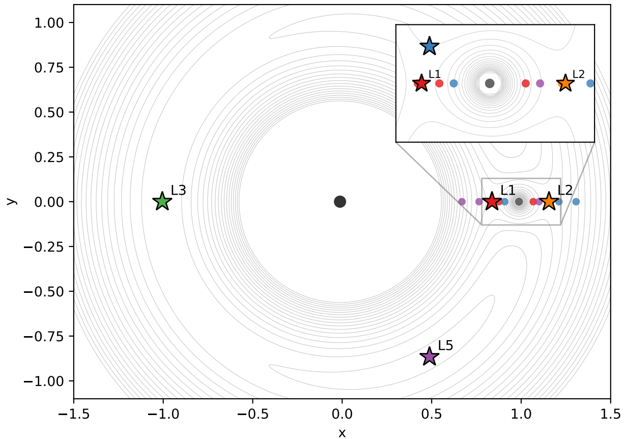
Trajectories of the curvature-learning machine (Earth-Moon) circles: structural-grid seeds; stars: discovered Lagrange points
