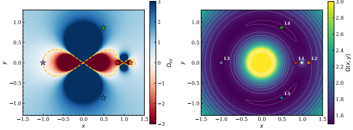
FIG. 1. Left: transverse curvature \Omega_{yy}(x, y) of the effective potential, Eq. (6), for the Earth–Moon mass ratio (red–blue, clipped at \pm 3 ). Red regions ( \Omega_{yy} < 0 ) are where the correction current activates ( \sigma = +1 , Eq. (12)); the dashed line is the contour \Omega_{yy} = 0 . Right: the effective potential \Omega(x, y) , Eq. (2). Stars mark the five Lagrange points; the three collinear ones lie in the red ( \Omega_{yy} < 0 ) saddle region, L_{4,5} in the blue region.
