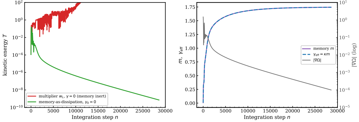
FIG. 2. Why the memory now computes, for one representative initial condition with no external damping. Left: kinetic energy T = \frac{1}{2}\|\dot{\mathbf{r}}\|^2 (log scale). Under the multiplier ansatz (7)–(9) with \gamma = 0 (red), T remains \mathcal{O}(1) and grows—the memory cannot dissipate (Proposition 1). Under memory-as-dissipation (13a)–(13d) with \gamma_0 = 0 (green), T \rightarrow 0 . Right: for the green run, the memory m (solid) and the damping \gamma_{\text{eff}} = \kappa m (dashed) ratchet up from zero and saturate, while the clause violation \|\nabla\Omega\| (grey, right axis) decays to the threshold.
