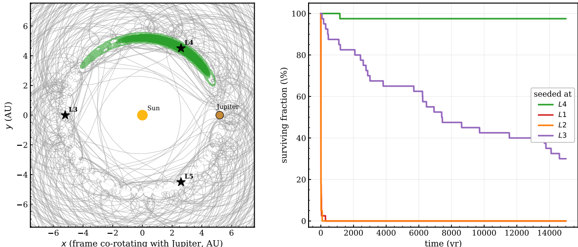
FIG. 4. Independent N -body stability cross-check (Sun–Jupiter). Left: a cloud seeded near L_4 in the frame co-rotating with Jupiter; green paths are surviving tadpole librations about L_4 , grey are escapees. Sun, Jupiter, and the L_3/L_4/L_5 points are marked. Right: surviving fraction vs. time for clouds seeded at L_4, L_1, L_2, L_3 . L_4 is stable; the collinear L_1, L_2 escape within one orbit; L_3 is also unstable but with a long e -folding time. No memory or correction current is used—this is pure gravitational integration.
