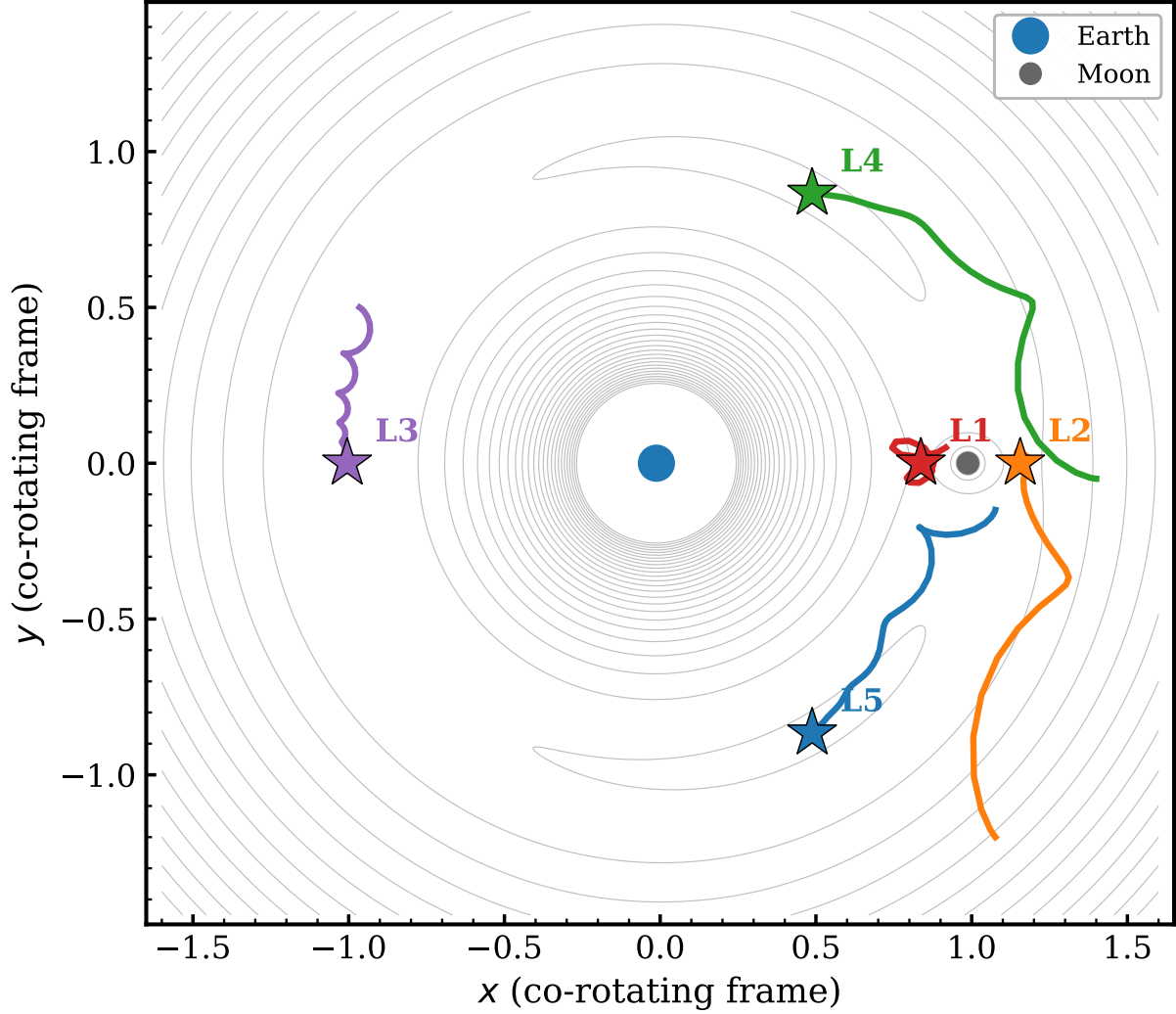
FIG. 3. Representative memory-as-dissipation trajectories for Earth–Moon ( \mu = 0.0121 ), one per Lagrange point, from a 10 \times 10 grid of starts. Grey curves: level sets of \Omega . Stars: the discovered equilibria. No solution coordinates are supplied to the integrator.
