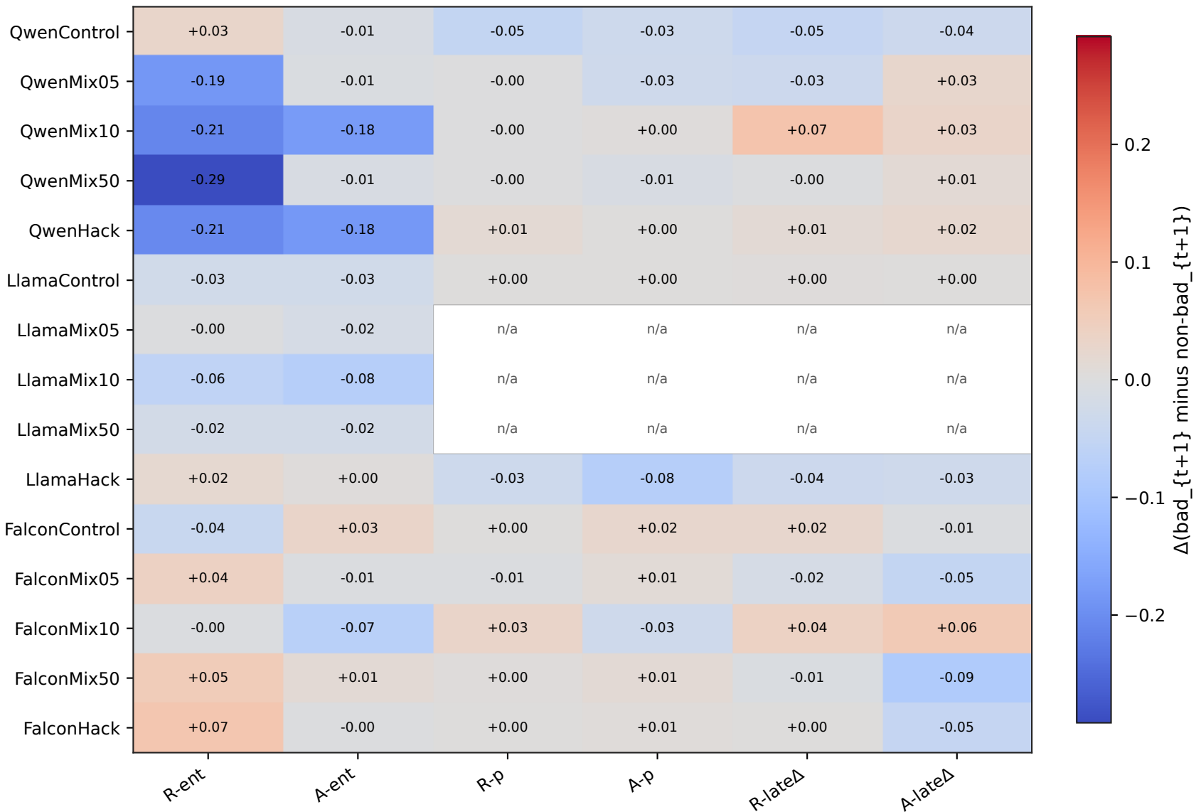
Appendix: signed next-step delta heatmap at TTC=32
