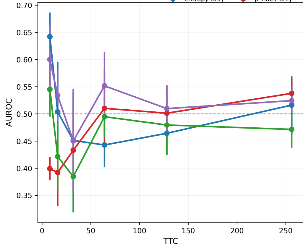
Qwen next-step prediction vs test-time compute
