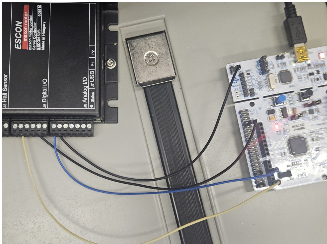
Figure 3.1: Physical command setup used for STM32-to-ESCON testing. The Nucleo board supplies only low-current command signals; motor power and velocity control remain handled by the ESCON.
