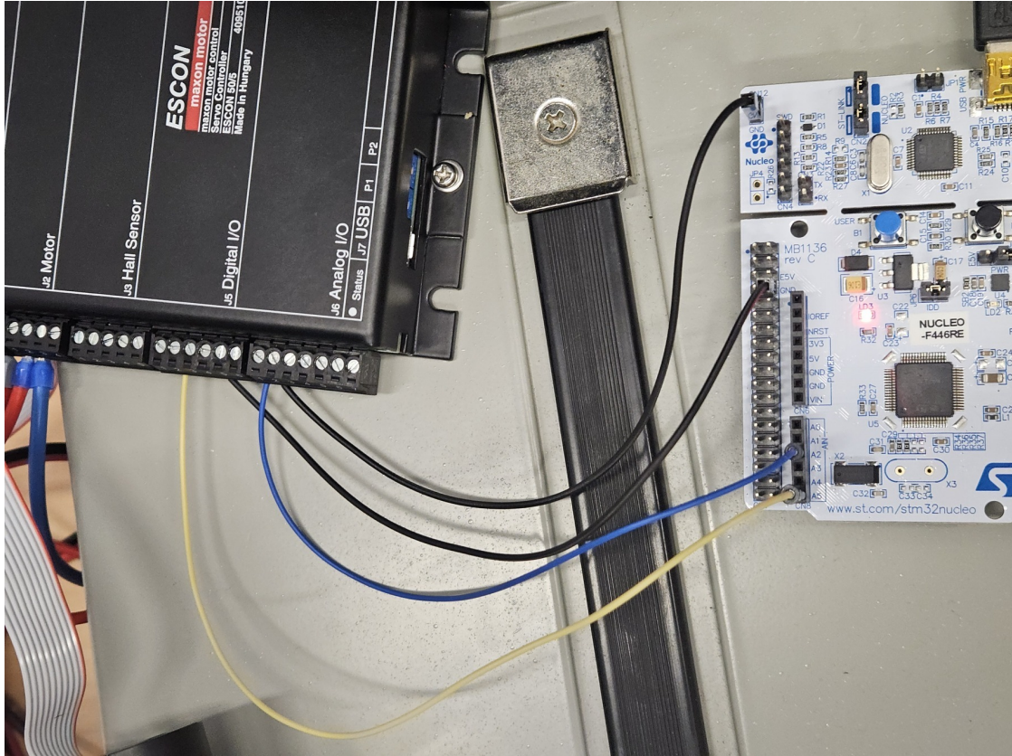
Figure 3.2: Observed STM32-to-ESCON signal wiring. The photograph documents the physical command interface, not a completed finger mechanism.
