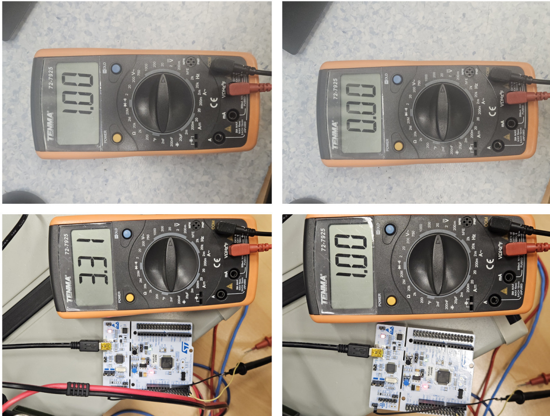
Figure 3.3: Voltage-isolation evidence from the STM32 debugging stage. The timed/blink test and button tests were used to confirm inactive and active command states before the ESCON inputs were connected.
