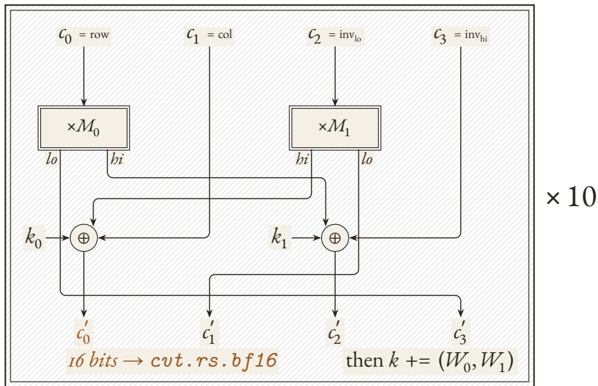
FIG. II. One round of Philox-4 \times 32 , unrolled ten times inside the epilogue.
