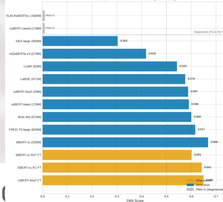
SAV Benchmark — PAN Scores (all models)
