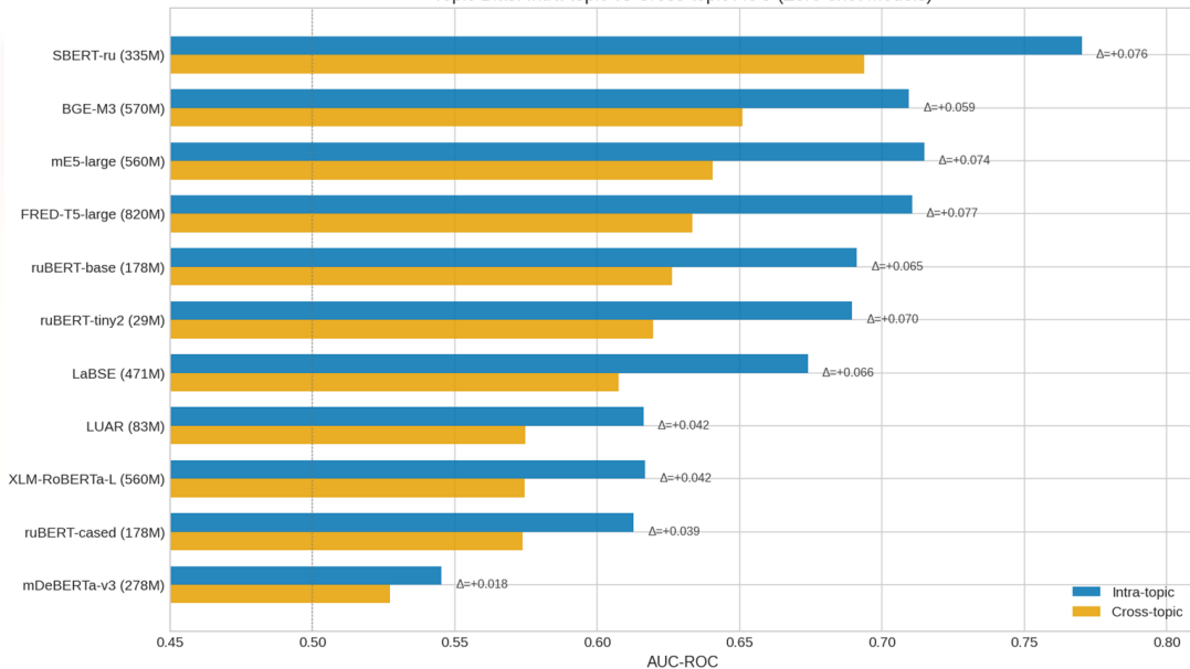
Topic Bias: Intra-topic vs Cross-topic AUC (Zero-shot Models)
