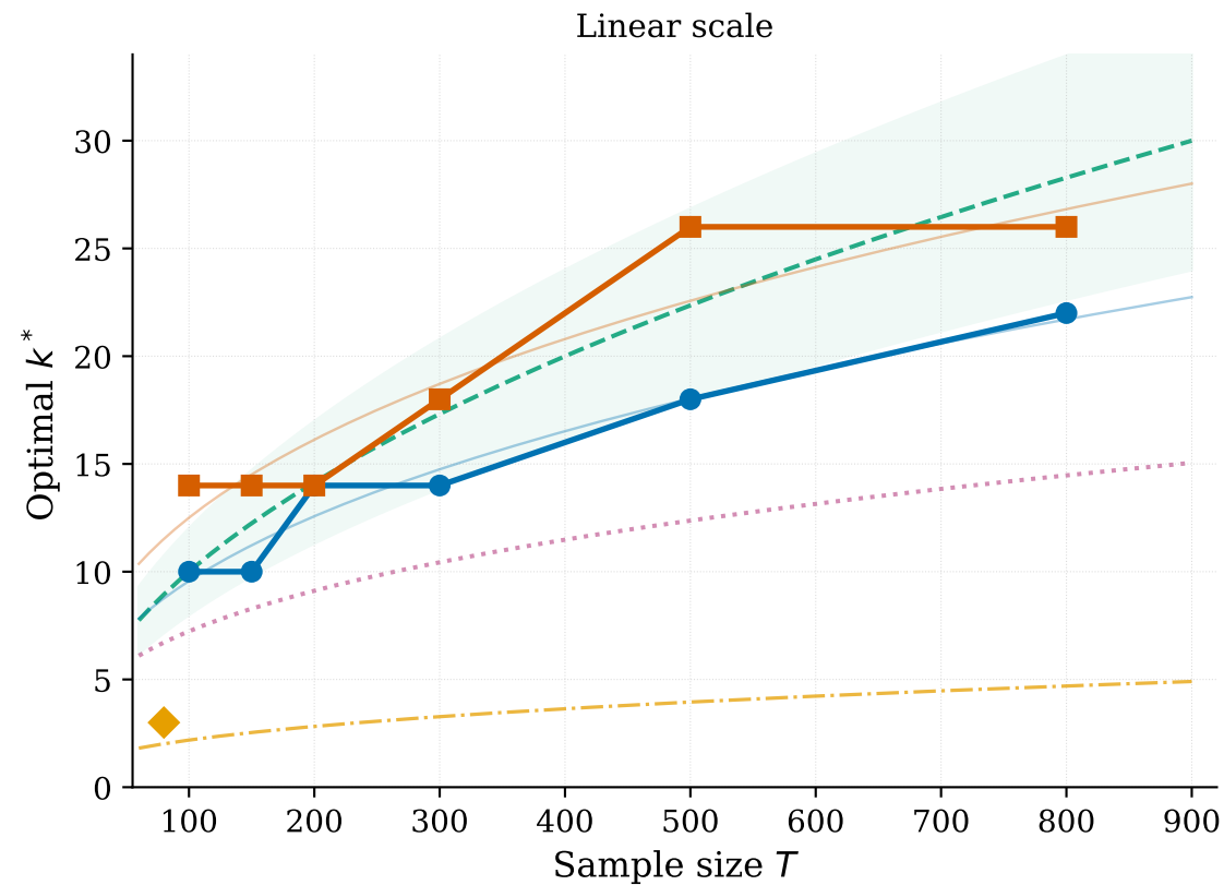
Optimal subset size k^* vs sample size T Endogenous cases: RMSFE minimiser ( m = 50, 500 MC reps); exogenous H = 6 : formula only (data pending)
