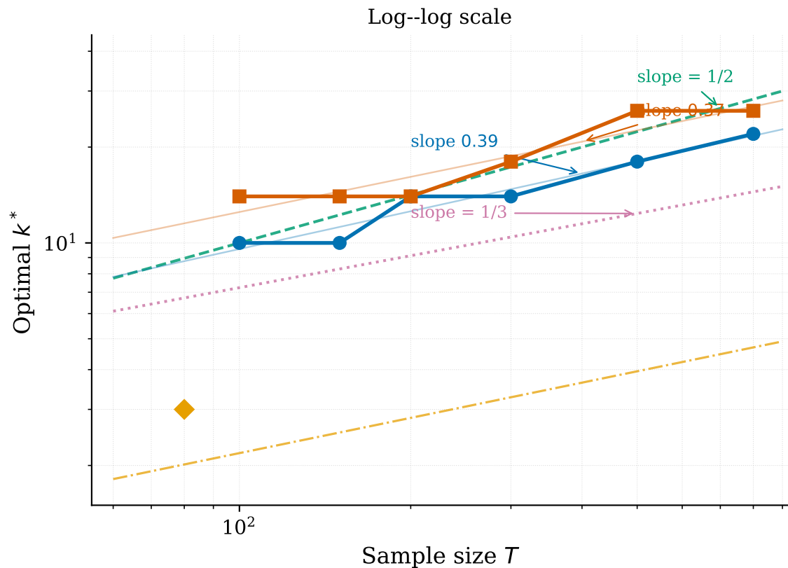
Optimal subset size k^* vs sample size T Endogenous cases: RMSFE minimiser ( m = 50, 500 MC reps); exogenous H = 6 : formula only (data pending)
