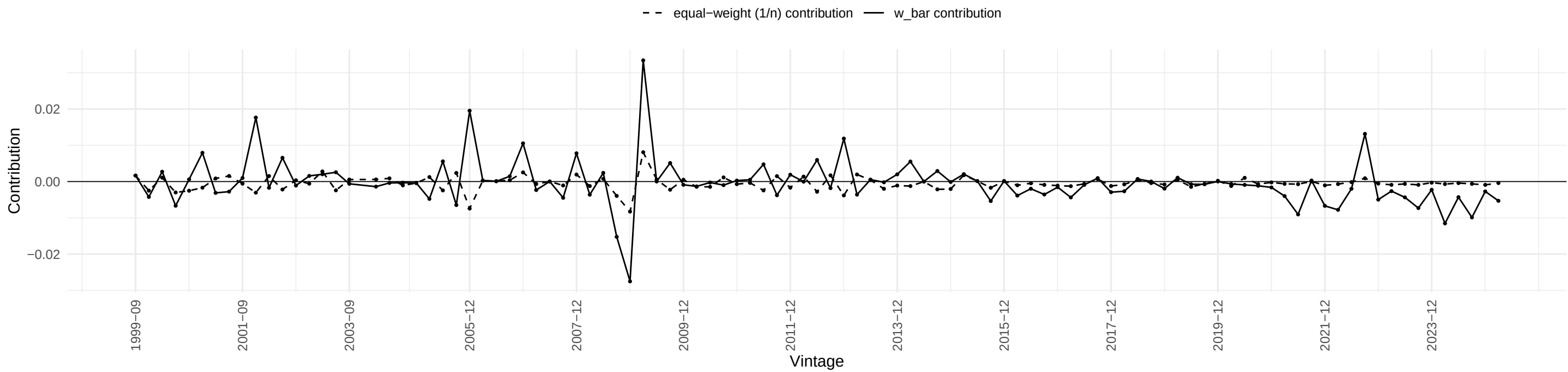
CUSR0000SAC – w_bar vs equal-weight contribution
