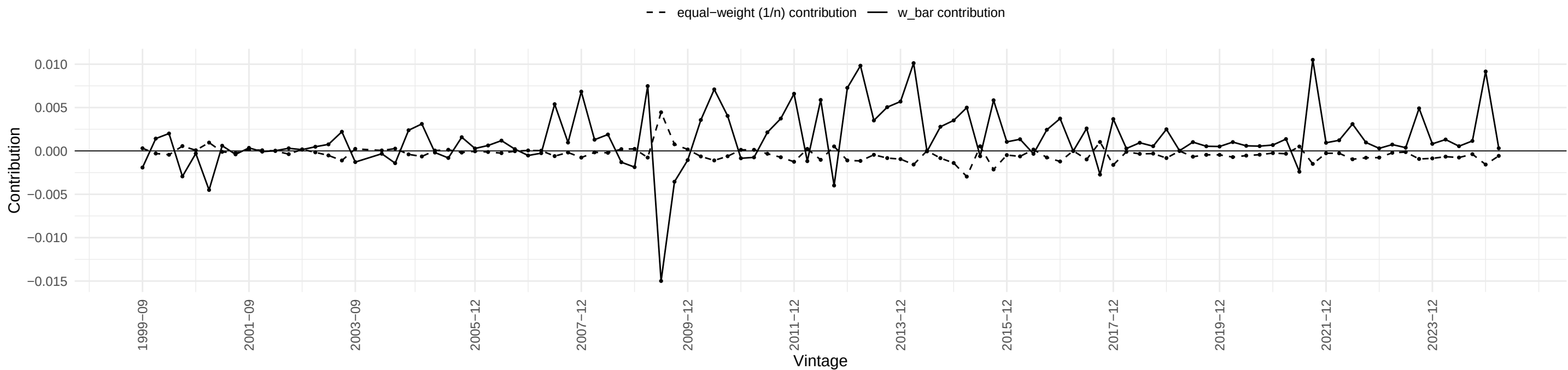
EXCAUSx – \bar{w} vs equal-weight contribution
