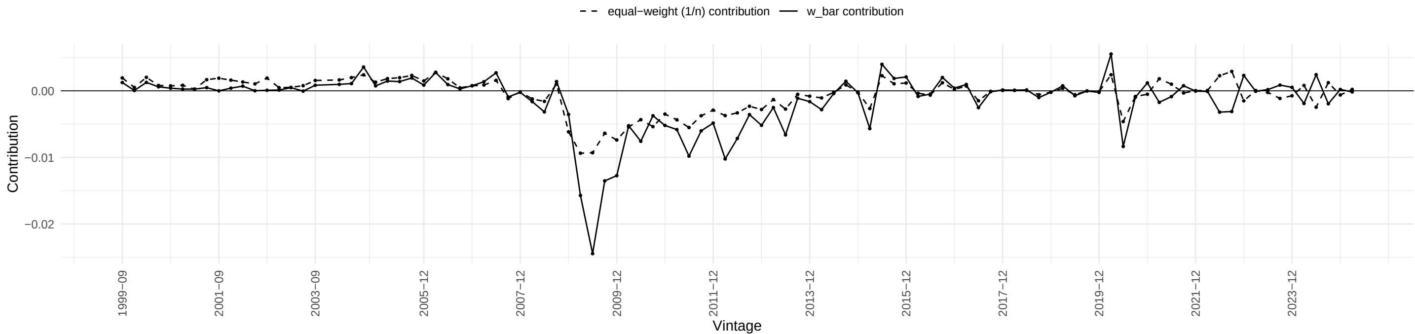
HOUSTNE – w_bar vs equal-weight contribution
