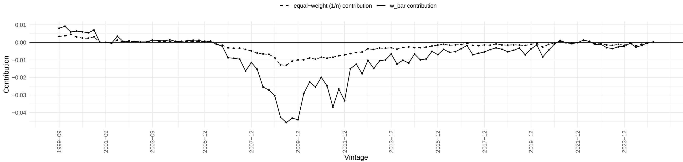
PERMITMW – w_bar vs equal-weight contribution
