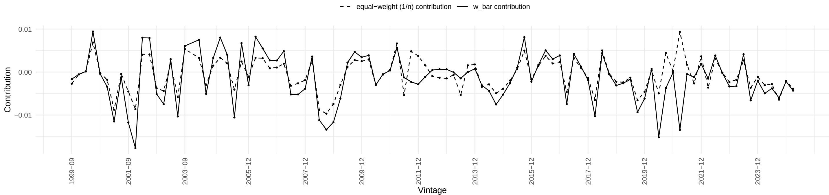
UEMPLT5 – w_{\text{bar}} vs equal-weight contribution
