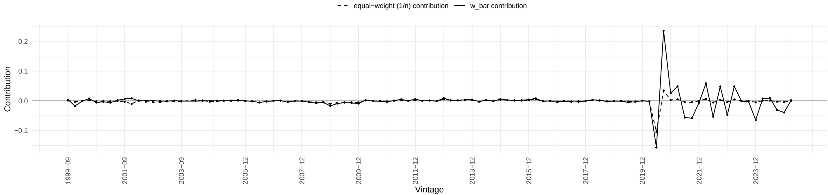
USTRADE – w_{\text{bar}} vs equal-weight contribution
