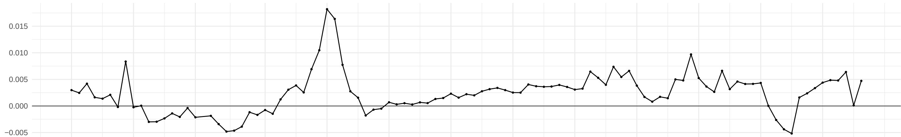
Contribution
