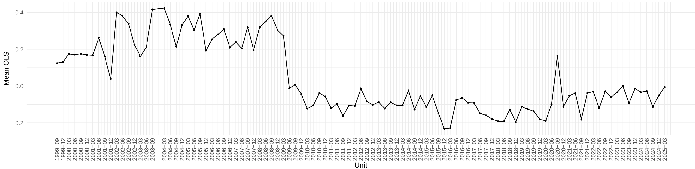
Evolution of AAA OLS coefficient across time
