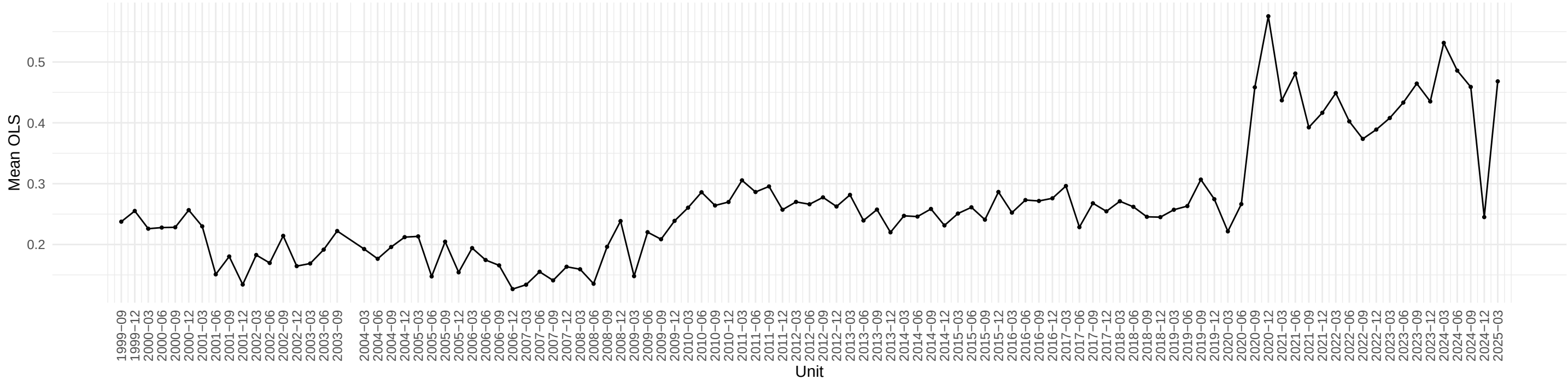
Evolution of AWOTMAN OLS coefficient across time
