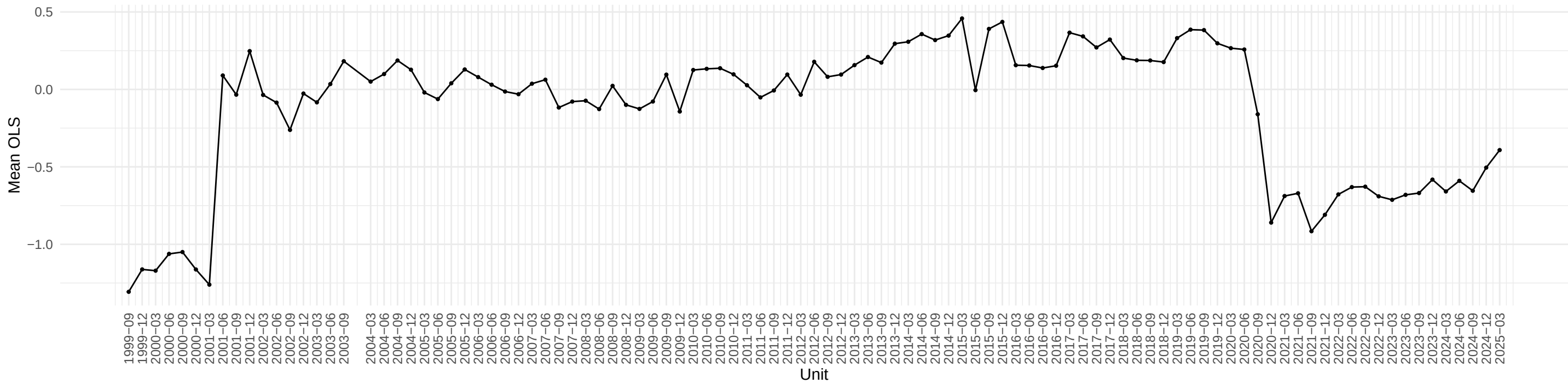
Evolution of CES2000000008 OLS coefficient across time
