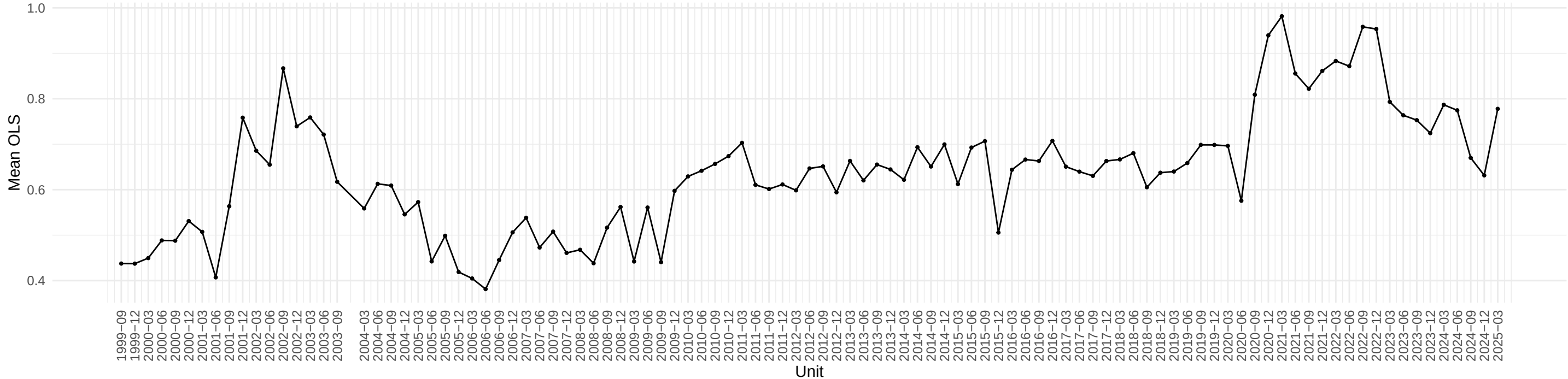
Evolution of CUMFNS OLS coefficient across time
