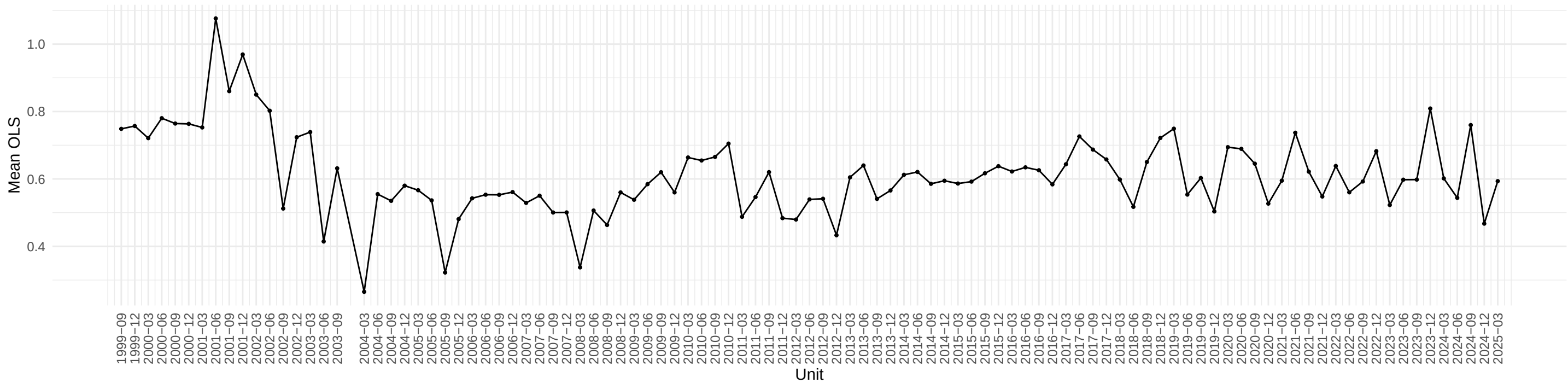
Evolution of DMANEMP OLS coefficient across time
