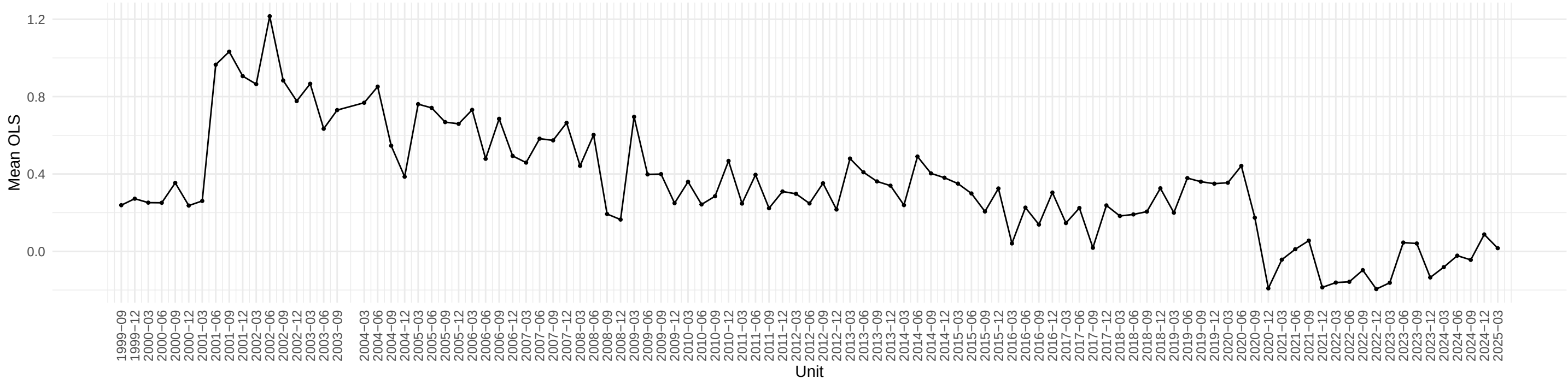
Evolution of GS1 OLS coefficient across time
