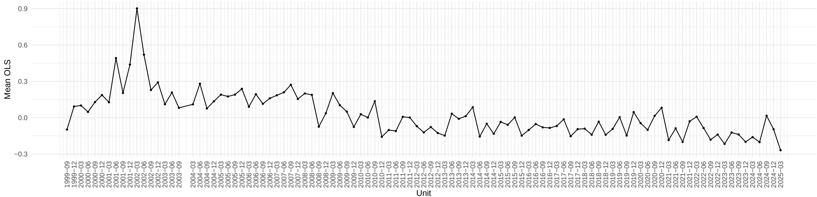
Evolution of GS5 OLS coefficient across time
