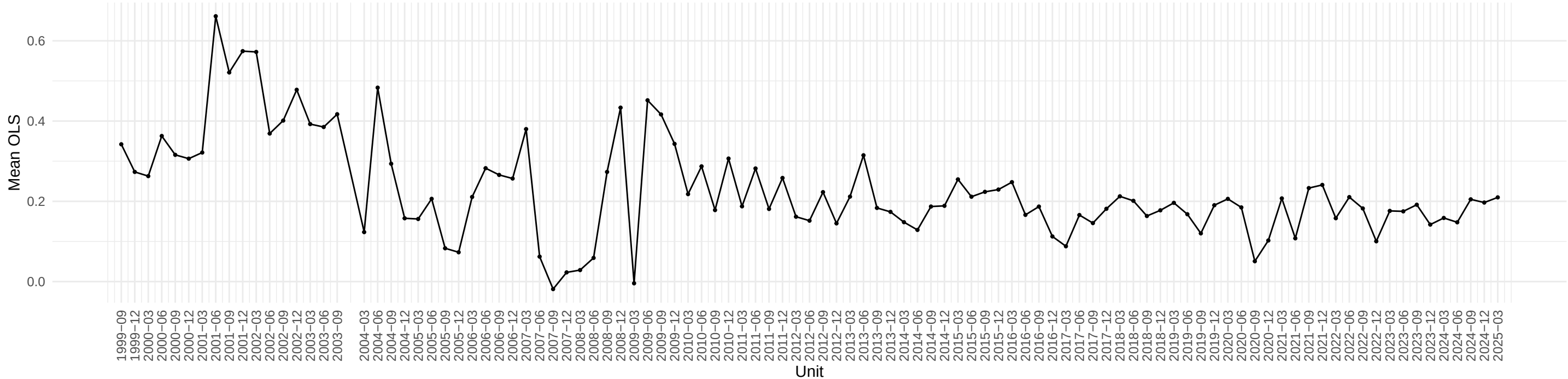
Evolution of HOUSTMW OLS coefficient across time
