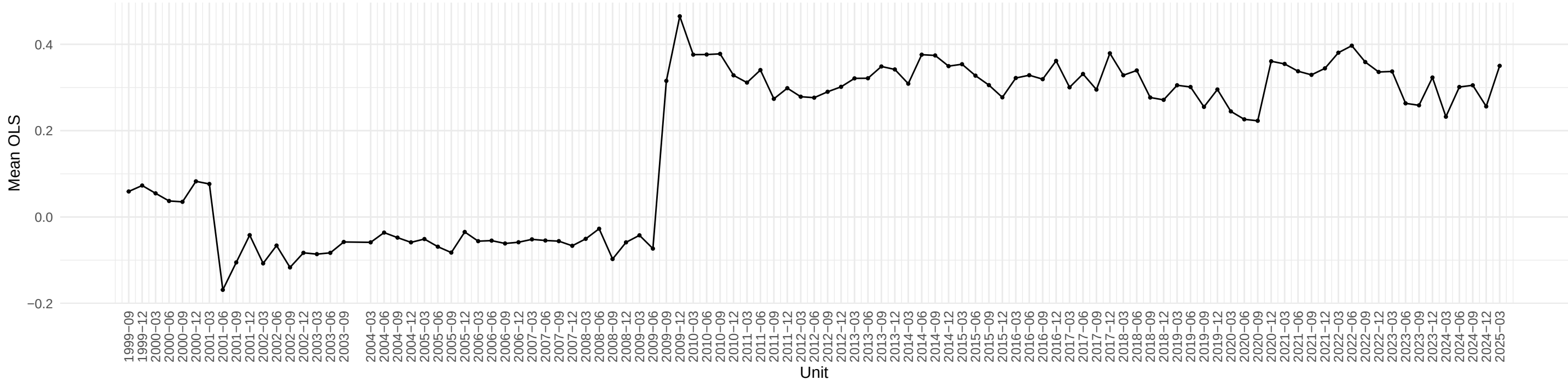
Evolution of INVEST OLS coefficient across time
